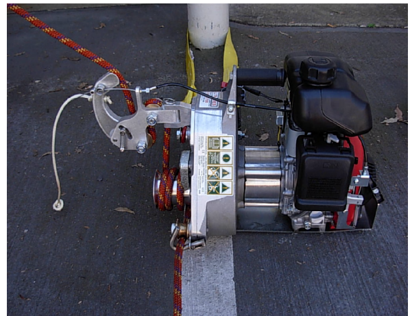
showing lifting version with brake and clutch
